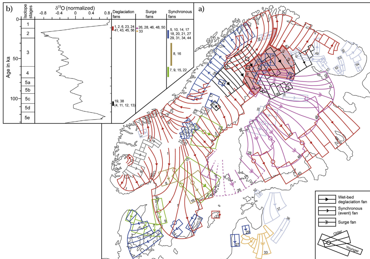
Fig. 4. Application of Kleman and Borgström's (1996) glacial inversion of flow-sets (fans) to the Fennoscandian Ice Sheet, from Kleman et al. (2006) . Different fan types are 'unfolded' to produce a time-slice sequence of ice sheet evolution that spans from 115 to 9 ka.
