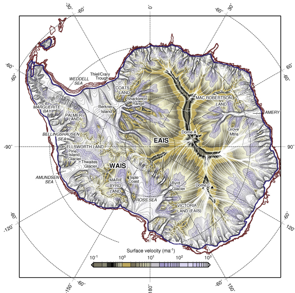
Fig. 15. Surface velocity pattern of the modelled glacial maximum configuration ice sheet, with flow-lines illustrating steady-state surface transport routes from Gollede et al. (2013).
