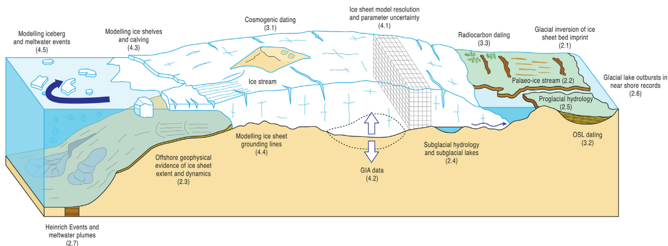
Fig. 1. Simple schematic of an ice sheet (not to scale) showing some of the key domains and approaches that are used to constrain the extent, thickness and dynamics of ice sheets at the regional to continental scale. Numbers in brackets refer to sub-sections in the manuscript where recent developments in each of these areas are discussed.
