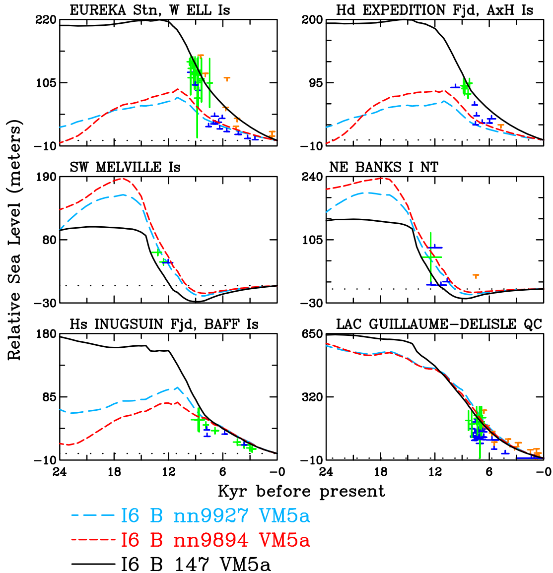
Fig. 13. Comparisons of Glacial Isostatic Adjustment-based (GIA-based) and data-calibrated glaciological ice sheet modelling-based predictions of relative sea level (RSL) histories at six example locations on the North American continent that were once covered by the Laurentide and Innuitian ice-sheets. The black lines are the predictions of the GIA-based model. The blue and red dashed curves are for glaciological ice sheet models nn9927 and nn9894, respectively (Tarasov et al., 2012). These six comparisons are not intended to be representative of the differences between the quality of these different predictions at the totality of available locations from this geographical region. The site codes corresponding to the six site names shown here are 1160 (Eureka Stn.), 1186 (Hd Expedition Fjd), 1254 (SW Melville Is), 1356 (NE Banks Is), 1434 (Hs Inugsuin Fjd) and 1632 (Lac Guillaume-Delisle). These locations are shown as red circles on Supplementary Fig. 1. A complete set of such comparisons is available in Supplementary Fig. 2, which are shown in blue circles on Supplementary Fig. 1.
