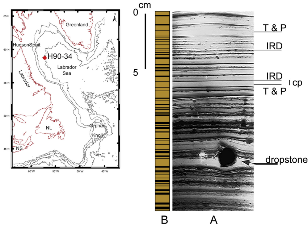
Fig. 10. Example of fine-scale structure within a Heinrich Layer from the Labrador Sea that can be several metres thick (modified from Hesse and Khodabakhsh, 1998). Left panel shows the location map. Right panel shows: (A) X-radiograph showing the rhythmic succession of individual IRD layers (dark) and turbidite and/or meltwater plume deposit layers (light). The existence of individual IRD laminae is possible only if there is enough time between the occurrences of the turbidity currents, otherwise the IRD would be incorporated in the turbidites as drop-stones or reworked by the turbidity currents. (B) a large number of light–dark couplets are identified over a 17 cm interval. Additional work is required to determine the average duration of a couplet, but it is likely that they are annual (T and P = turbidites and meltwater plume deposits; IRD = ice rafted debris; cp = couplet).
