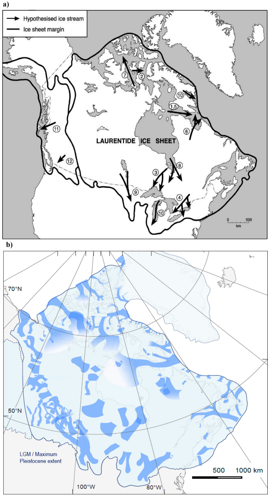
Fig. 5. The number of hypothesized ice streams has grown rapidly over recent years, with those in the Laurentide Ice Sheet increasing from 10 (black arrows) that were reviewed by Stokes and Clark (2001) in (a), to over 100 (blue shading) in the latest inventory compiled by Margold et al. (2015) in (b).
