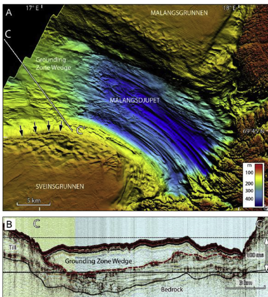
Fig. 6. (a) Multi-beam bathymetric data showing a submarine palaeo-ice stream bed (ice flow bottom right to top left) in Malangsdjupet, northern Norway (from Ottesen et al., 2008). This cross-shelf trough exhibits many of the geomorphological criteria for identifying palaeo-ice streams (Stokes and Clark, 1999), including a convergent onset zone feeding into a main trunk characterised by mega-scale glacial lineations with abrupt lateral margins and ice stream shear margin moraines (black arrows); (b) Seismic data across the grounding zone wedge (100 m s = ~90 m on the vertical axis).
