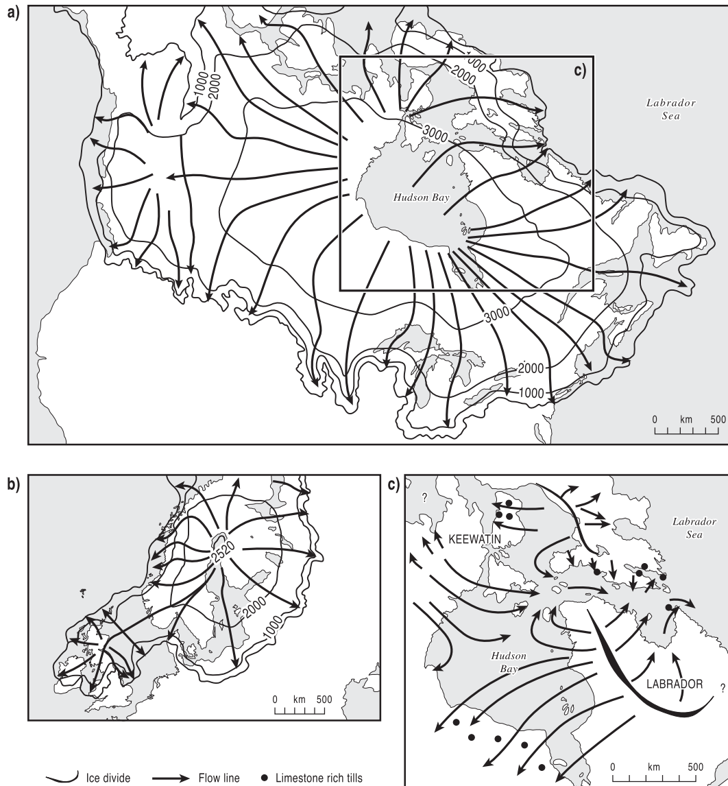
Fig. 2. Map of modelled ice thickness (metres) and flow-lines of the North American (a) and Eurasian Ice Sheets (b) after Denton and Hughes (1981). Andrews (1982) noted the mismatch between the single-domed ice sheet configurations and flow patterns inferred from till stratigraphy and erratic dispersal data (e.g. Shilts, 1980), shown in (c). Figures redrawn from Andrews (1982).
