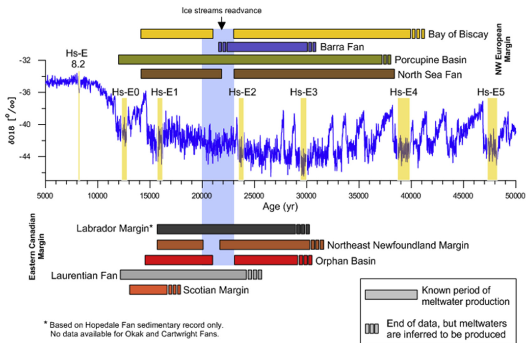
Fig. 11. Major meltwater and iceberg (IRD) events from the Laurentide and Eurasian Ice Sheets from 50 to 5 ka (Hs-E = Hudson Strait events). Compilation based on sedimentation rates from Skene and Piper (2003), Lekens et al. (2005, 2006), Piper et al. (2007), Toucanne et al. (2009), Tripsanas and Piper (2008a,b), Scourse et al. (2009), Haapaniemi et al. (2010), Saint-Ange and Piper (2011) and Roger et al. (2013). Different coloured bars for meltwater production emphasise that each source has a distinctive detrital petrology.
