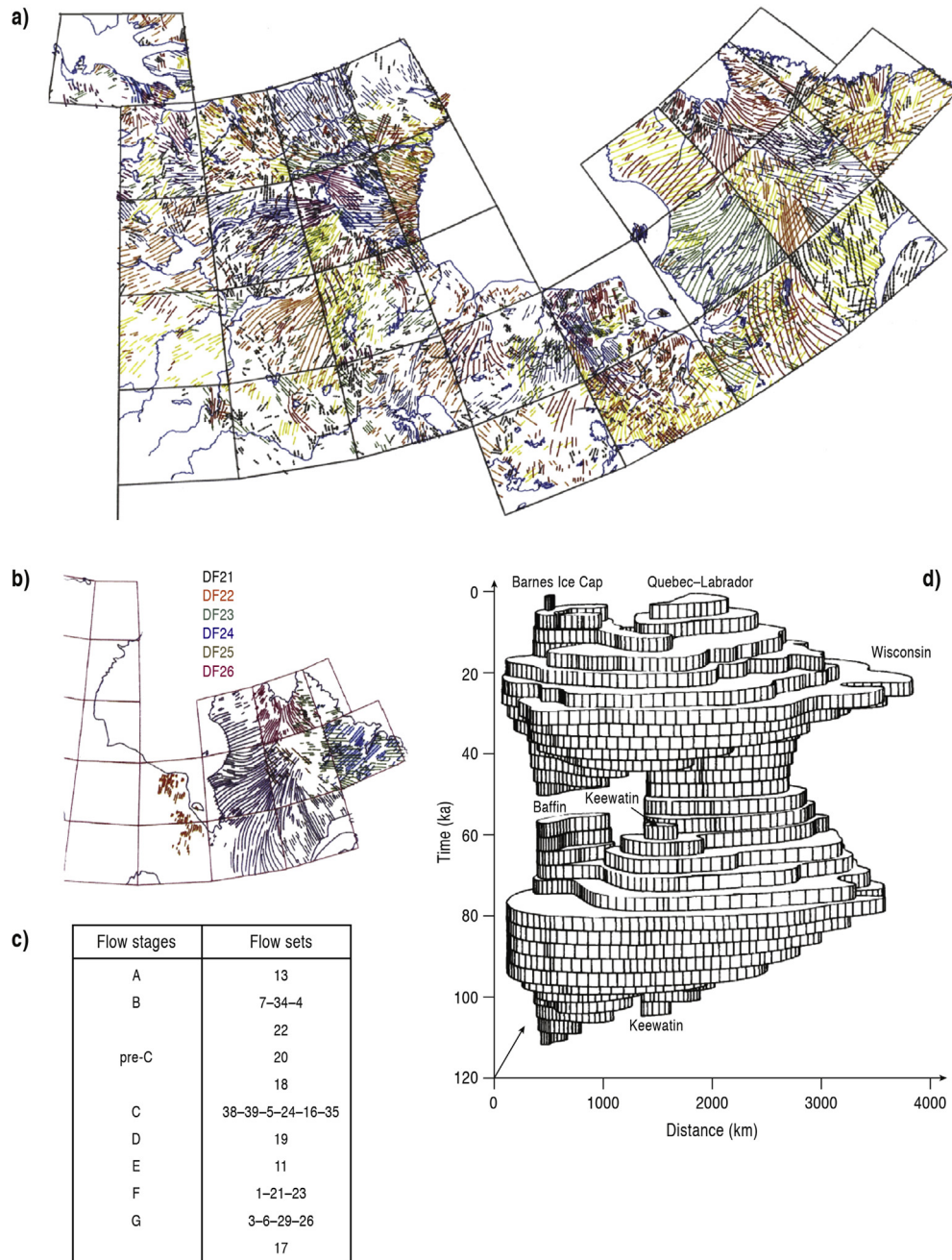
Fig. 3. (a) Multiple cross-cutting flow-sets (colours used arbitrarily to show different flow-sets) from the central part of the Laurentide Ice Sheet mapped by Boulton and Clark (1990b), including close-up in (b). These flow-sets are numbered (e.g. DF21, DF22 in (b)) and stacked into relative age sequence (flow-stages) (c) using cross-cutting relationships, and reveal a highly mobile ice sheet reconstruction, which shows the areal extent of the ice sheet through time in (d). Figures redrawn from Boulton and Clark (1990b).
