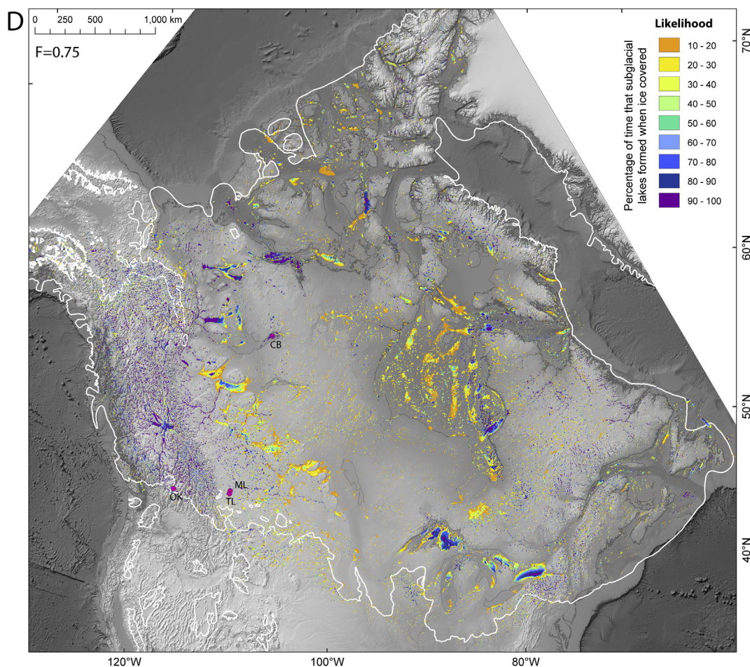
Fig. 8. Modelled subglacial lake likelihood map for the North American Ice Sheet Complex from 32 to 6 ka from Livingstone et al. (2013). F is the flotation criteria which is the ratio of non-local, subglacial water pressure to ice overburden pressure (i.e., if F = 1 , the water pressure is at the ice-overburden pressure). White line shows ice extent from Dyke et al. (2002). Pink circles refer to published palaeo-subglacial lake records: CB = Christie Bay, Great Slave Lake; ML = McGregor Lake; TL = Travers Lake; OK = Okanagon.
