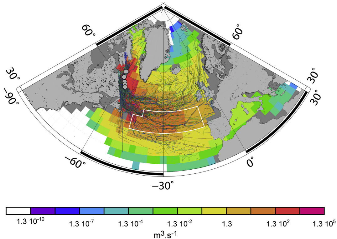
Fig. 14. Simulated freshwater input and iceberg tracks in a Last Glacial Maximum climate simulated Heinrich event with interactive icebergs (from Jongma et al., 2013). The colour scale indicates the freshwater flux input to the ocean in \text{m}^3 \text{s}^{-1} due to melting icebergs (note logarithmic scale). The five grey circles show the chosen fixed input locations for the iceberg delivery. The coloured lines are a sample of iceberg tracks generated by the iceberg model. The white line in the centre shows the area classically chosen for 'Ruddiman belt' freshwater hosing experiments for comparison with the coloured area at the background.
