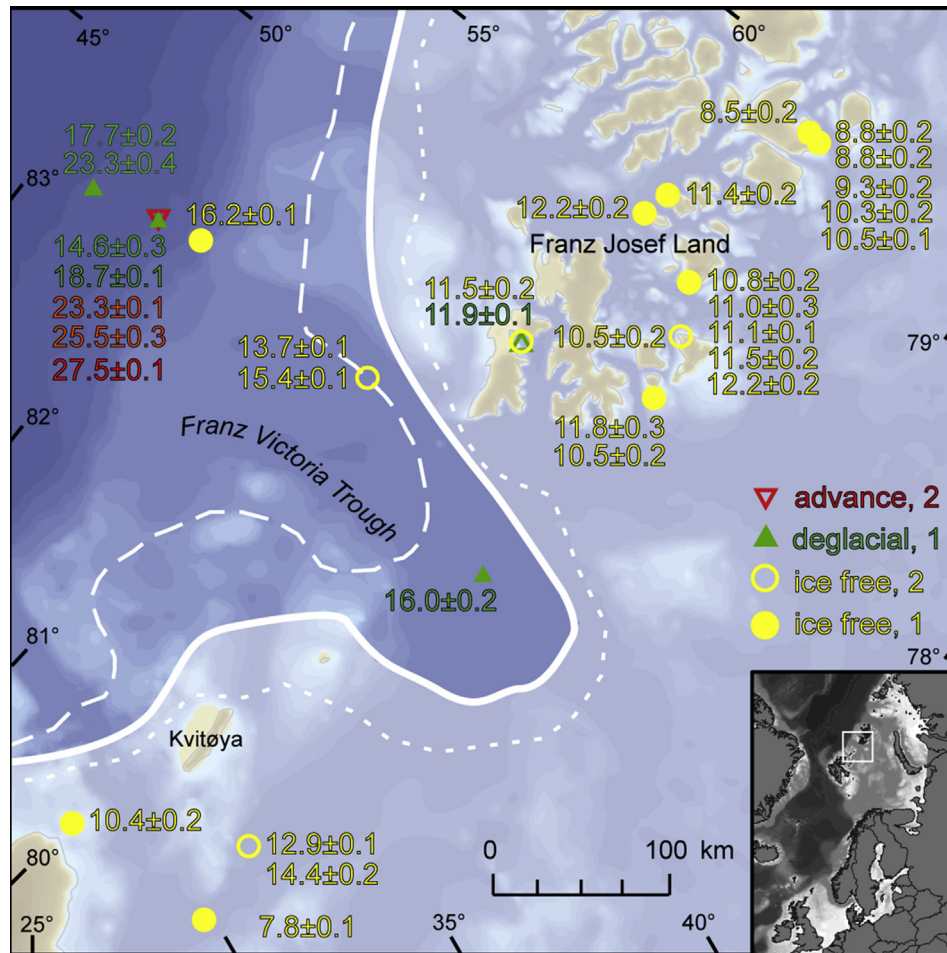
Fig. 12. Excerpt from the DATED-1 ice margin reconstruction (Hughes et al., 2015) for 16 ka, east of Svalbard, showing ice margin positions interpolated between available dates. Maximum (dashed white line), most credible (solid white line) and minimum (dotted white line) ice margin positions are shown. Date sites and age labels (ka) are coloured by glacial classification (after Hughes et al., 2011): advance (e.g. below till; red); deglacial (e.g. above till; green); ice free (e.g. no stratigraphic information available; light green). Dates are considered reliable are shown by solid symbols (e.g. 1), dates that may be reliable are shown in outline (e.g. 2).
