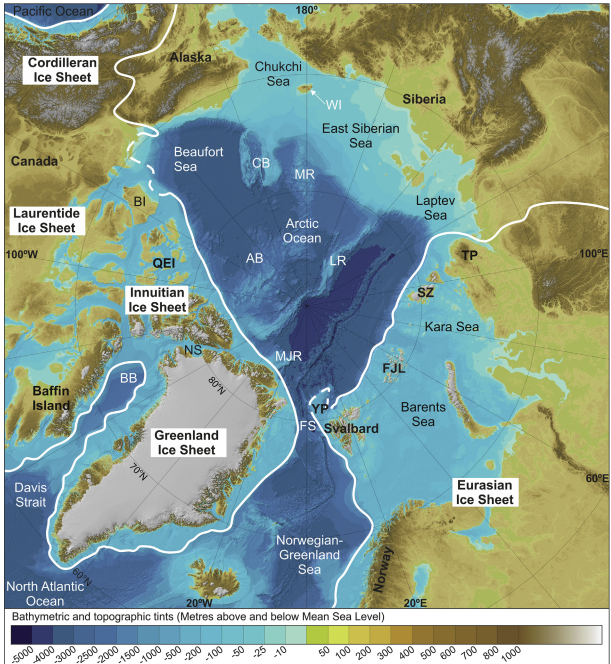
Fig. 7. Maximum Quaternary extent (white line; dashed in areas of uncertainty) of the Eurasian (MIS 6: Svendsen et al., 2004), Greenland (MIS 2: Ehlers and Gibbard, 2004), Innuitian and Laurentide (MIS 2: Dyke et al., 2002), and Cordilleran ice sheets (Pleistocene maximum from Manley and Kaufman, 2002) in the high Arctic from Batchelor and Dowdeswell (2014) displayed on IBCAO bathymetric data (Jakobsson et al., 2012), with place names (WI = Wrangel Island; MR = Mendeleev Ridge; SZ = Severnaya Zemlya; FJL = Franz Josef Land; YP = Yermak Plateau; FS = Fram Strait; MJR = Morris Jesup Rise; NS = Nares Strait; QEI = Queen Elizabeth Islands; BB = Baffin Bay; CB = Chukchi Borderland; LR = Lomonosov Ridge). Figure modified from Batchelor and Dowdeswell (2014).
