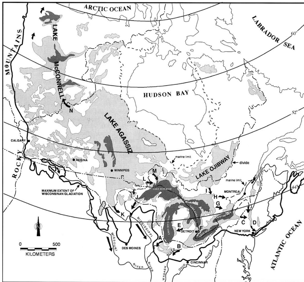
Fig. 9. Total area covered by large proglacial lakes in North America (grey) during the last retreat of the LIS (from Teller, 2004, Fig. 1, after Teller, 1987). Major continental divides shown by dash-dot lines. Names of the major lakes are shown in the region where they formed. Major overflow routes from lakes are shown by arrows; letters identify their names as follows: A = Chicago outlet, B = Wabash River Valley, C = Mohawk Valley, D = Hudson Valley, E = Grand River Valley, F = Port Huron outlet, G = Fenelon Falls outlet, H = North Bay outlet, I = Temiskaming outlet, J = Duluth outlet, K = Minnesota River Valley, L = Kaminiskwia outlet, M = eastern Agassiz outlets, N = Clearwater outlet. Extent of proglacial lakes in Hudson Bay Lowland and St. Lawrence Lowland are not shown where lacustrine sediments are now buried by marine sediment.
